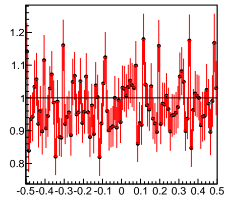
Localx in FPIX -252
