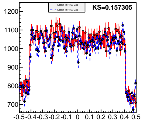
Localx in FPIX 115
