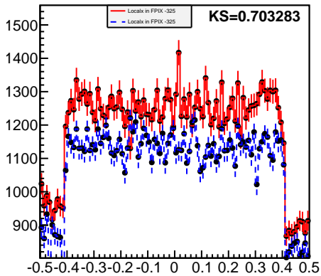
Localx in FPIX -050
