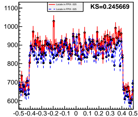
Localx in FPIX -325
