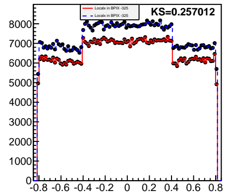
Localx in BPIX 253
