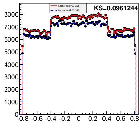
Localx in BPIX -050
