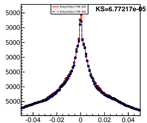
Entry-Exity in TIB -325
