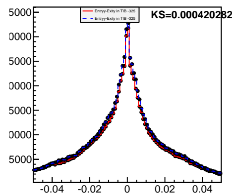
Entry-Exity in TIB -151
