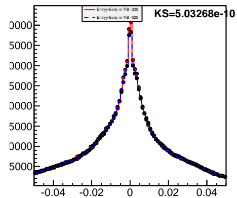
Entry-Exity in TIB 115
