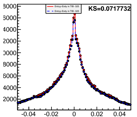
Entry-Exity in TIB -252
