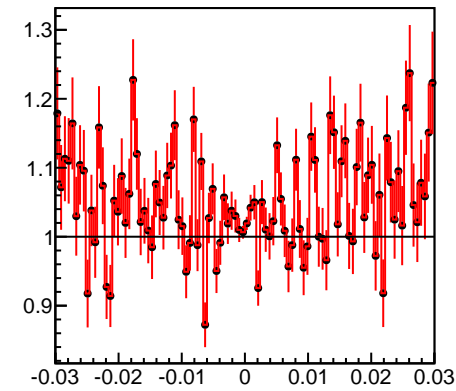
Entry-Exit in BPIX -252
