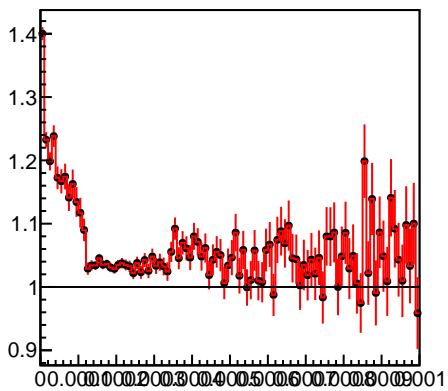
Energy loss in TOB -215
