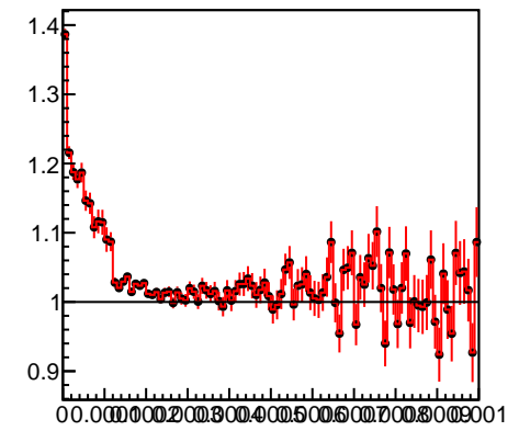
Energy loss in TOB 115
