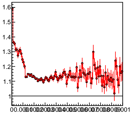
Energy loss in TOB 152
