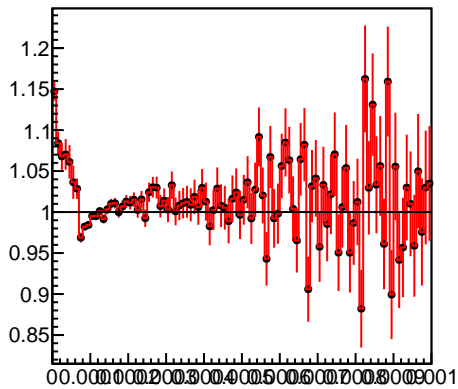
Energy loss in TIB -105
