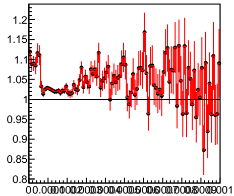
Energy loss in TIB -325
