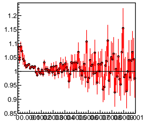
Energy loss in TIB 115
