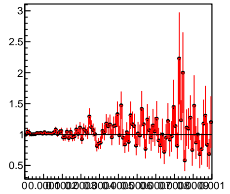
Energy loss in FPIX 115
