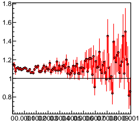
Energy loss in BPIX 152
