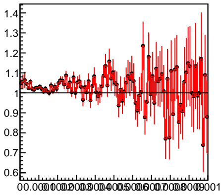
Energy loss in BPIX -215
