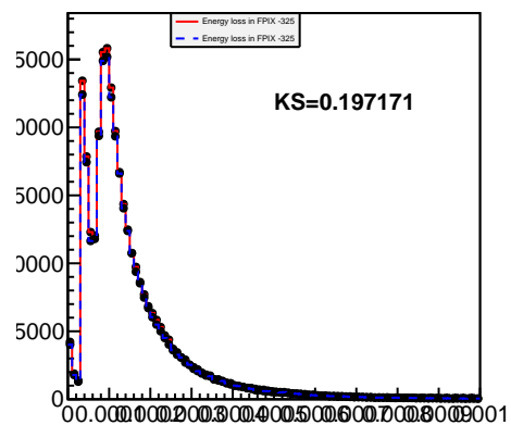
Energy loss in BPIX -215
