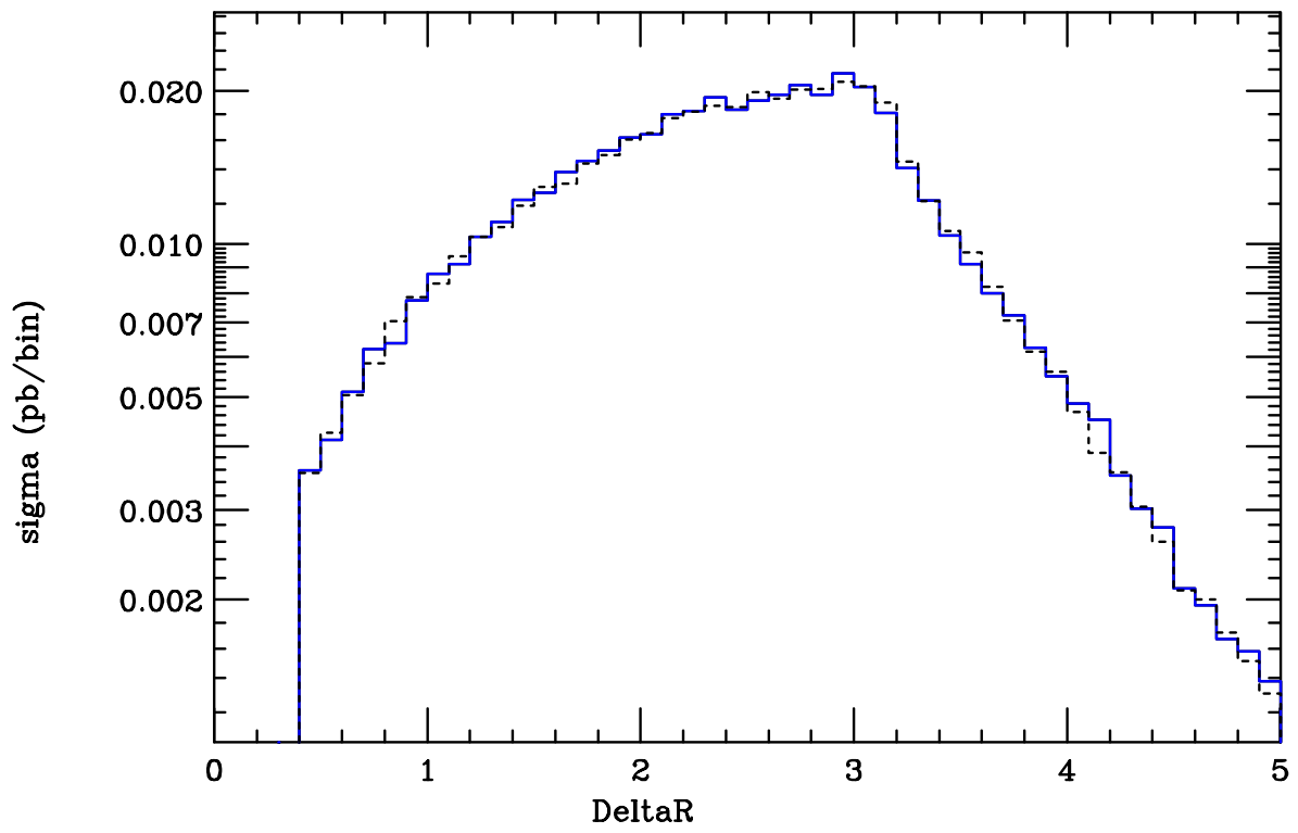
R(jet2,e+1)
