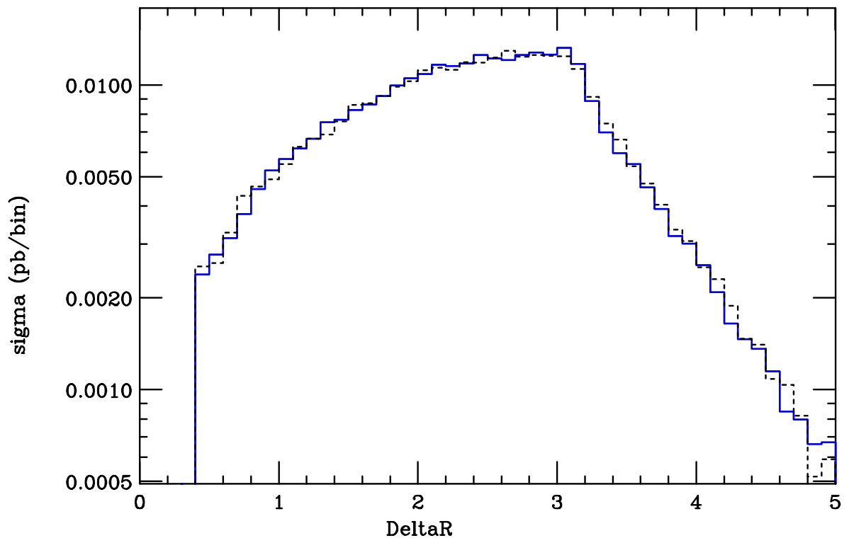
R(jet2,e-1)
