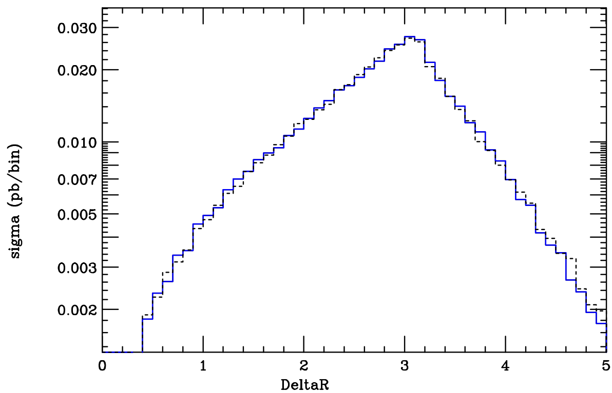
R(jet1,e+1)
