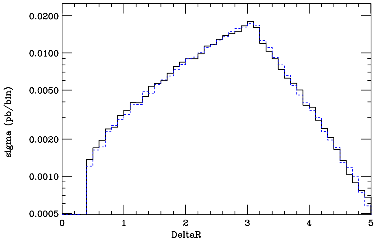
R(jet1,e-1)
