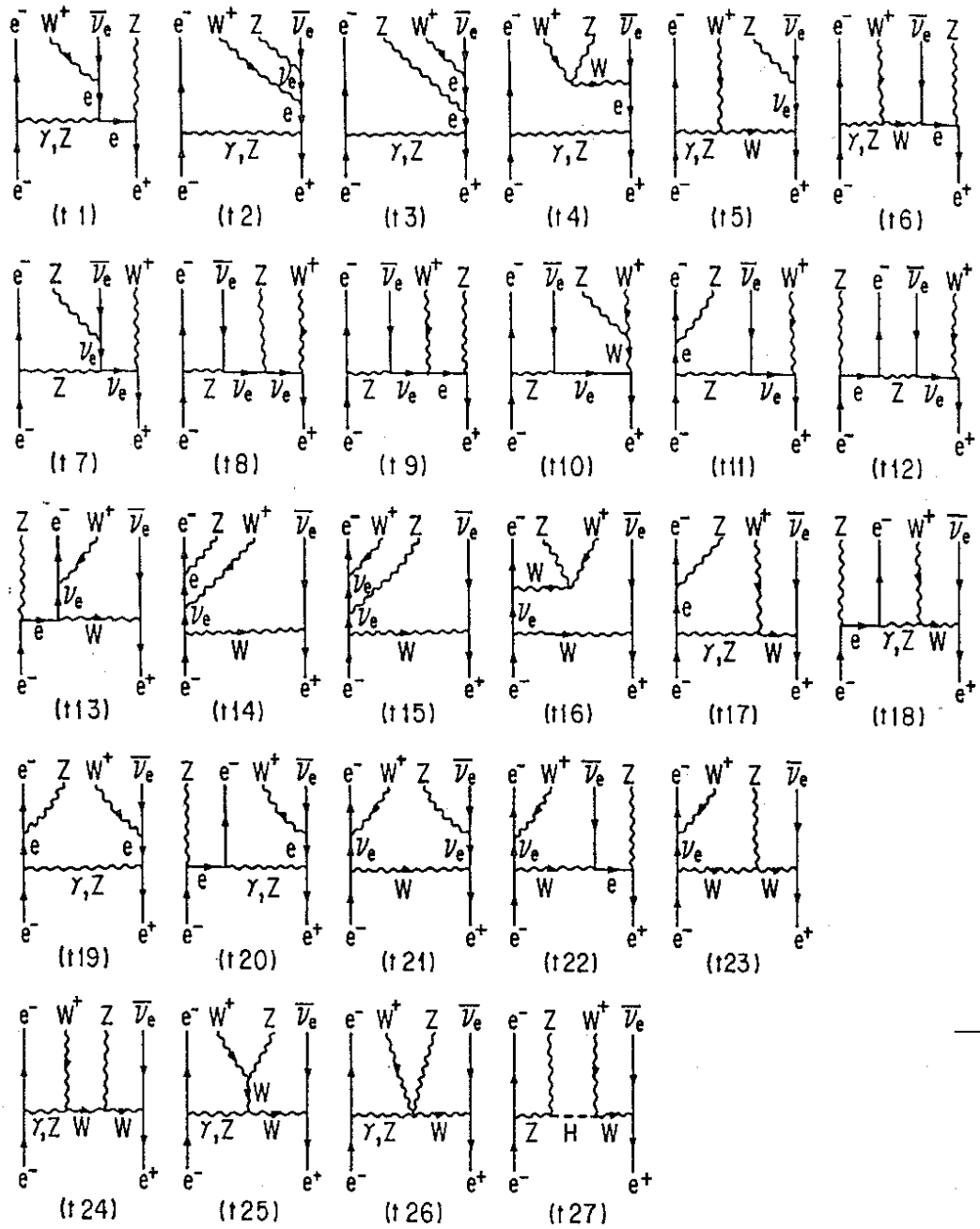
Figure 15: Feynman diagrams for the process e^-e^+ \rightarrow e^-\bar{\nu}_e W^+ Z . Only the t -channel diagrams are shown.
