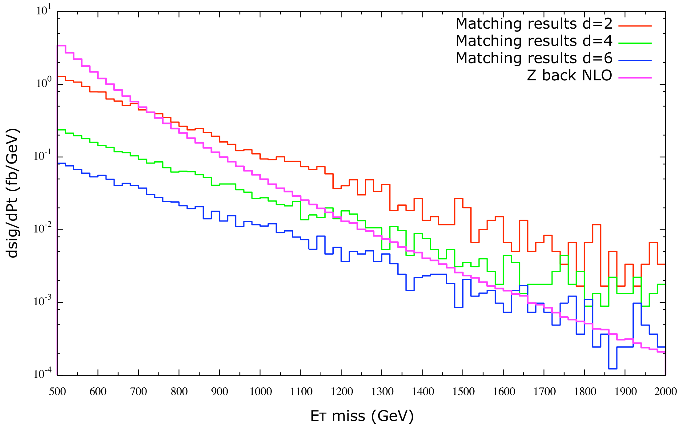
Missing ET distribution for ADD with M_s = 5 TeV
