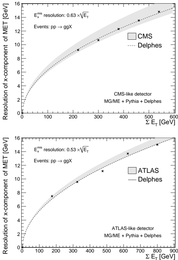
Figure 10: \sigma(E_x^{\text{mis}}) as a function on the scalar sum of all towers ( \Sigma E_T ) for pp \rightarrow gg events, for a CMS-like detector (top) and an ATLAS-like detector (bottom), for di-jet events produced with MADGRAPH/MADEVENT and hadronised with PYTHIA.
