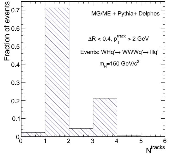
Figure 6: Distribution of the number of tracks N^{\text{tracks}} within a small jet cone for true \tau -jets, normalised to unity. Photoproduced WH events, where W bosons decay leptonically ( e, \mu, \tau ), as in Fig. 5. Histogram entries correspond to true \tau -jets, matched with generator-level data.
