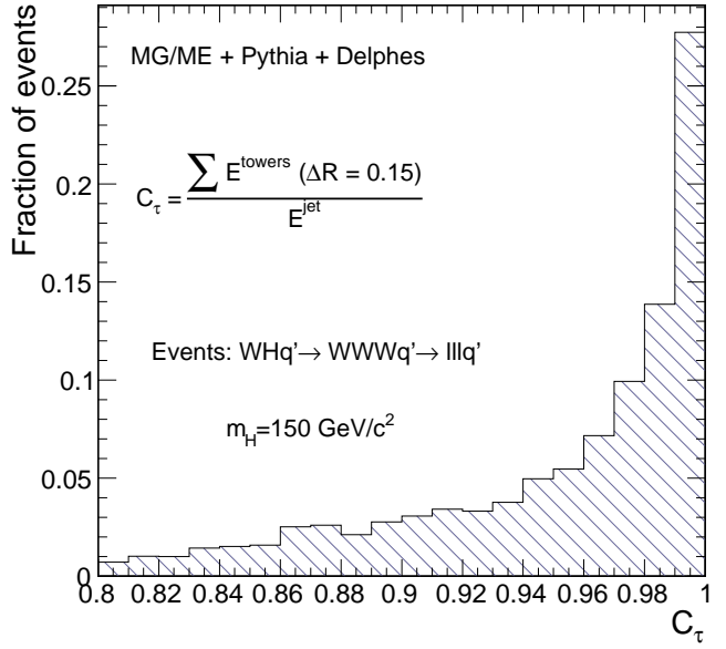
Figure 5: Distribution of the electromagnetic collimation C_\tau variable for true \tau -jets, normalised to unity. This distribution is shown for associated WH photoproduction [17], where the Higgs boson decays into a W^+W^- pair. Each W boson decays into a \ell\nu_\ell pair, where \ell = e, \mu, \tau . Events generated with MadGraph/MadEvent [18]. Final state hadronisation is performed by Pythia [19]. Histogram entries correspond to true \tau -jets, matched with generator-level data.
