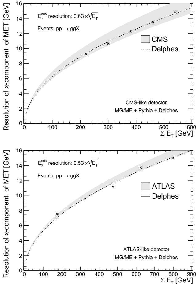
Figure 10: \sigma(E_x^{\text{mis}}) as a function on the scalar sum of all cells ( \Sigma E_T ) for pp \rightarrow gg events, for a CMS-like detector (top) and an ATLAS-like detector (bottom), for di-jet events produced with MadGraph/MadEvent and hadronised with Pythia .
