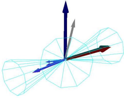
Figure 12: Example of pp(\gamma p \rightarrow Wt)pY event display in transverse view, with t \rightarrow Wb . One W boson decays into a \mu\nu_\mu pair and the second one into a e\nu_e pair. The surviving proton leaves a forward hemisphere with no hadronic activity. The isolated muon is shown as the dark blue vector. Around the electron, in red, is reconstructed a fake \tau -jet (blue cone surrounding a green arrow). The reconstructed missing energy is visible in grey.
