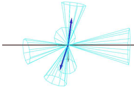
Figure 13: Example of inclusive gluon pair production pp \rightarrow ggX . Many jets are present in the event, in particular along the beam axis (black line).
