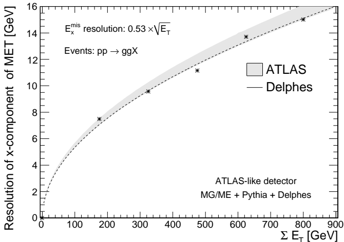
Figure 10: \sigma(E_x^{\text{mis}}) as a function on the scalar sum of all cells ( \Sigma E_T ) for pp \rightarrow gg events, for a CMS-like detector (top) and an ATLAS-like detector (bottom), for di-jet events produced with MadGraph/MadEvent and hadronised with Pythia .
