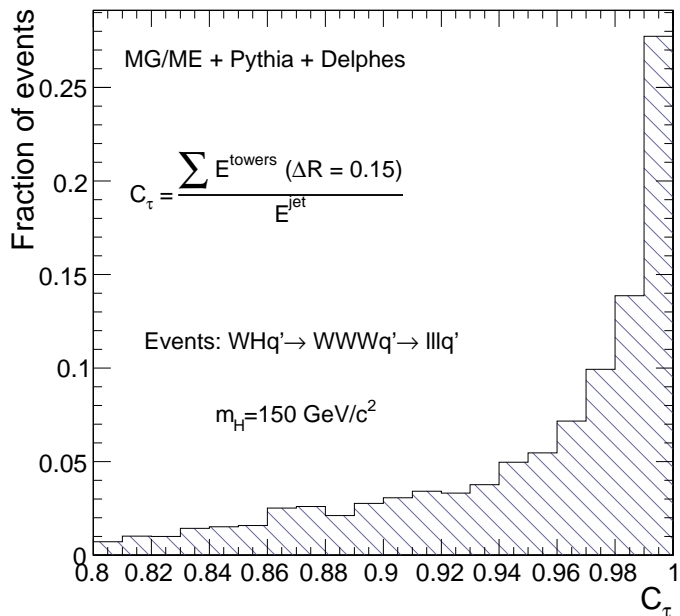
Figure 5: Distribution of the electromagnetic collimation C_\tau variable for true \tau -jets, normalised to unity. This distribution is shown for associated WH photoproduction [19], where the Higgs boson decays into a W^+W^- pair. Each W boson decays into a \ell\nu_\ell pair, where \ell = e, \mu, \tau . Events generated with MadGraph/MadEvent [20]. Final state hadronisation is performed by Pythia [21]. Histogram entries correspond to true \tau -jets, matched with generator-level data.
