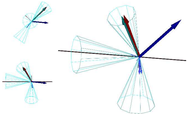
Figure 12: Example of pp(\gamma p \rightarrow Wt)pX event display in different orientations, with t \rightarrow Wb . One W boson decays into a \mu\nu_\mu pair and the second one into a e\nu_e pair. The surviving proton leaves a forward hemisphere with no hadronic activity. The isolated muon is shown as the dark blue vector. Around the electron, in red, is reconstructed a fake \tau -jet (green vector surrounded by a blue cone), while the reconstructed missing energy (in grey) is very small. One jet is visible in one forward region, along the beamline axis, opposite to the direction of the escaping proton.
