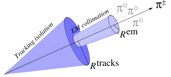
Figure 4: Illustration of the identification of \tau -jets (1-prong). The jet cone is narrow and contains only one track. The small cone serves to apply the electromagnetic collimation , while the broader cone is used to reconstruct the jet originating from the \tau -decay.
