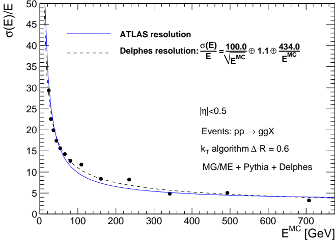
Figure 9: Relative energy resolution of reconstructed jets as a function of the energy of the closest jet of generator-level particles E^{MC} , in an ATLAS-like detector. The jets are reconstructed with the k_T algorithm with a radius R = 0.6 . The maximal matching distance between MC- and reconstructed jets is \Delta R = 0.2 . Only central jets are considered ( |\eta| < 0.5 ). Dotted line is the fit result for comparison to the ATLAS resolution [8], in blue. The pp \rightarrow gg di-jet events have been generated with MADGRAPH/MADEVENT and hadronised with PYTHIA.
