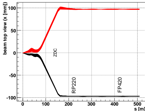
Figure 4: Default location of the very forward detectors, including ZDC, RP220 and FP420 in the LHC beamline. Incoming (beam 1, red) and outgoing (beam 2, black) beams on one side of the fifth interaction point (IP5, s = 0 m on the plot). The Zero Degree Calorimeter is located in perfect alignment with the beamline axis at the interaction point, at 140 m, the beam paths are separated. The forward taggers are near-beam detectors located at 220 m and 420 m. Beamline simulation with HECTOR [9].
