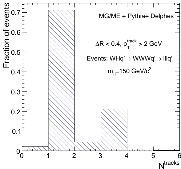
Figure 7: Distribution of the number of tracks N^{\text{tracks}} within a small jet cone for true \tau -jets, normalised to unity. Photoproduced WH events, where W bosons decay leptonically ( e, \mu, \tau ), as in Fig. 6. Histogram entries correspond to true \tau -jets, matched with generator-level data.
