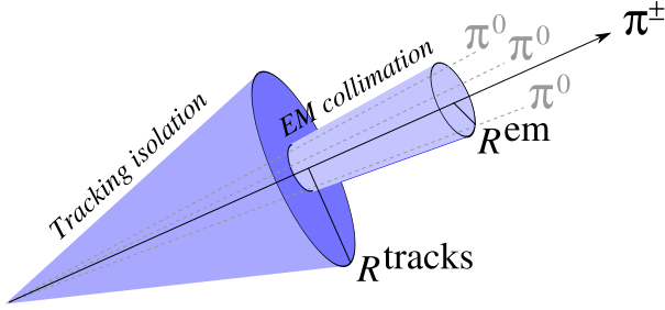
Figure 5: Illustration of the identification of \tau -jets (1-prong). The jet cone is narrow and contains only one track. The small cone serves to apply the electromagnetic collimation , while the broader cone is used to reconstruct the jet originating from the \tau -decay.
