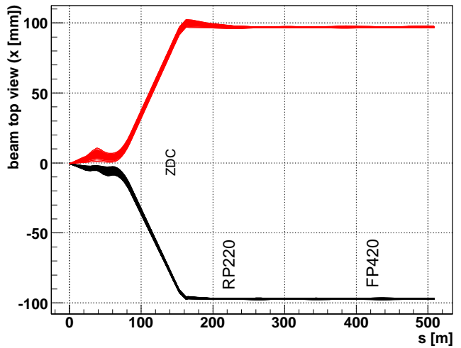
Figure 4: Default location of the very forward detectors, including ZDC and FP420 in the LHC beamline. Incoming (red) and outgoing (black) beams on one side of the interaction point ( s = 0 m). The Zero Degree Calorimeter is located in perfect alignment with the beamline axis at the interaction point, at 140 m, the beam paths are separated. The forward taggers are near-beam detectors located at 220 m and 420 m. Beamline simulation with HECTOR [9].
