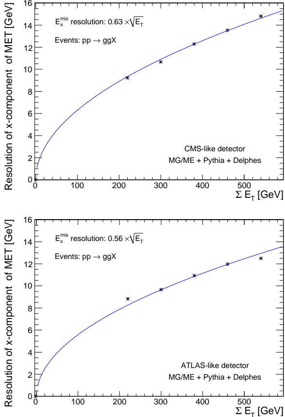
Figure 10: \sigma(E_x^{\text{miss}}) as a function on the scalar sum of all towers (\Sigma E_T) for pp \rightarrow gg events, for a CMS-like detector (top) and an ATLAS-like detector (bottom), for di-jet events produced with MADGRAPH/MADEVENT and hadronised with PYTHIA.
