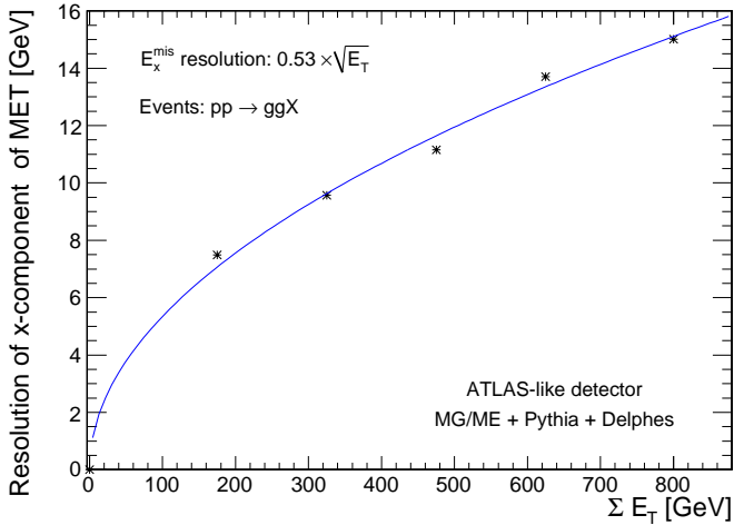
Figure 10: \sigma(E_x^{\text{miss}}) as a function on the scalar sum of all towers ( \Sigma E_T ) for pp \rightarrow gg events, for a CMS-like detector (top) and an ATLAS-like detector (bottom), for di-jet events produced with MADGRAPH/MADEVENT and hadronised with PYTHIA.
