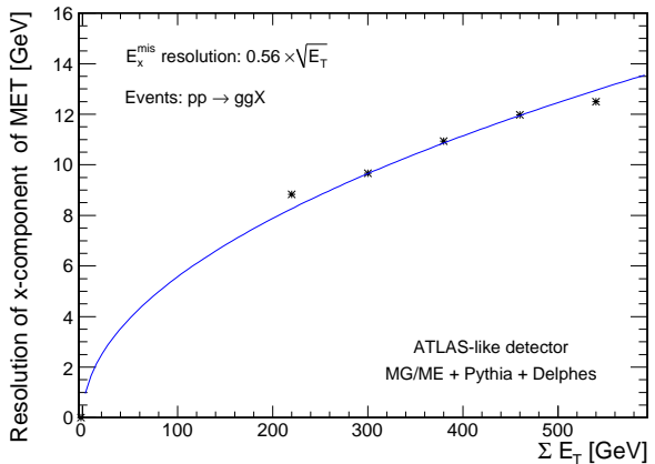
Figure 9: \sigma(E_x^{\text{mis}}) as a function on the scalar sum of all towers ( \Sigma E_T ) for pp \rightarrow gg events, for a CMS-like detector (top) and an ATLAS-like detector (bottom), for dijet events produced with MadGraph/MadEvent and hadronised with Pythia.
