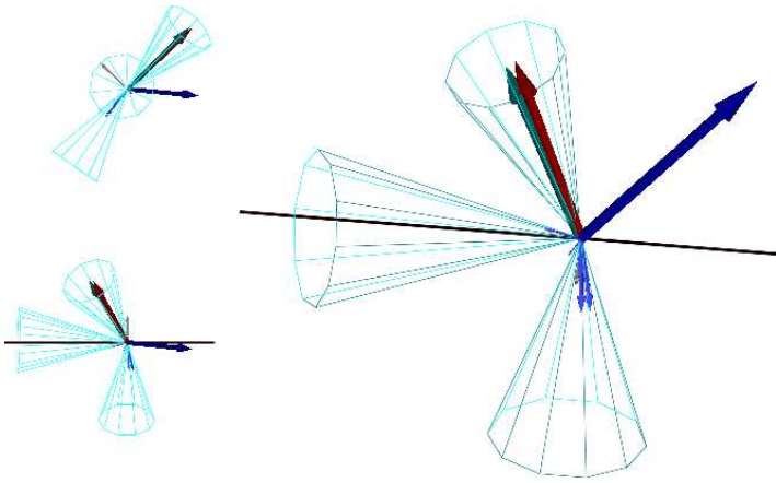
Figure 11: Example of pp(\gamma p \rightarrow Wt)pY event display in different orientations, with t \rightarrow Wb . One W boson decays into a \mu\nu_\mu pair and the second one into a e\nu_e pair. The surviving proton leaves a forward hemisphere with no hadronic activity. The isolated muon is shown as the dark blue vector. Around the electron, in red, is reconstructed a fake \tau -jet (green vector surrounded by a blue cone), while the reconstructed missing energy (in grey) is very small. One jet is visible in one forward region, along the beamline axis, opposite to the direction of the escaping proton.
