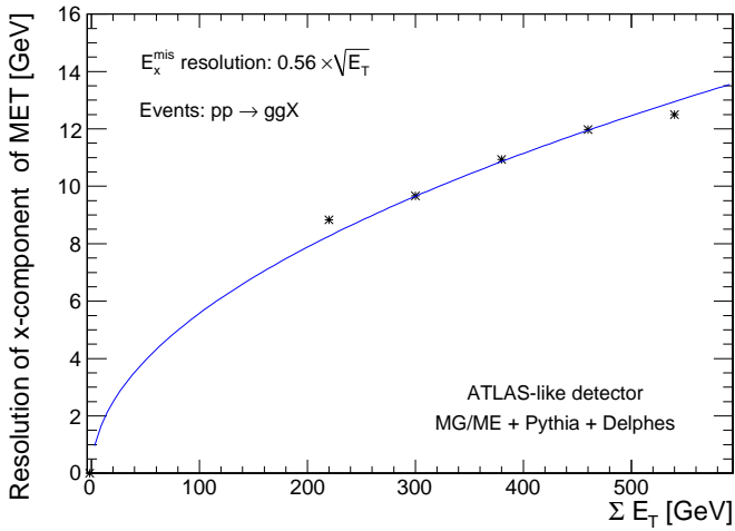
Figure 9: \sigma(E_x^{\text{mis}}) as a function on the scalar sum of all towers ( \Sigma E_T ) for pp \rightarrow gg events, for a CMS-like detector (top) and an ATLAS-like detector (bottom), for dijet events produced with MadGraph/MadEvent and hadronised with Pythia.
