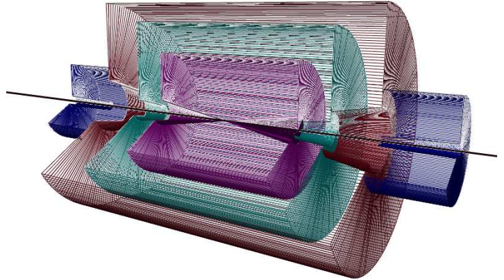
Figure 10: Layout of the generic detector geometry assumed in DELPHES. Open 3D-view of the detector with solid volumes. Same colour codes as for Fig. 2 are applied. Additional forward detectors are not depicted.
