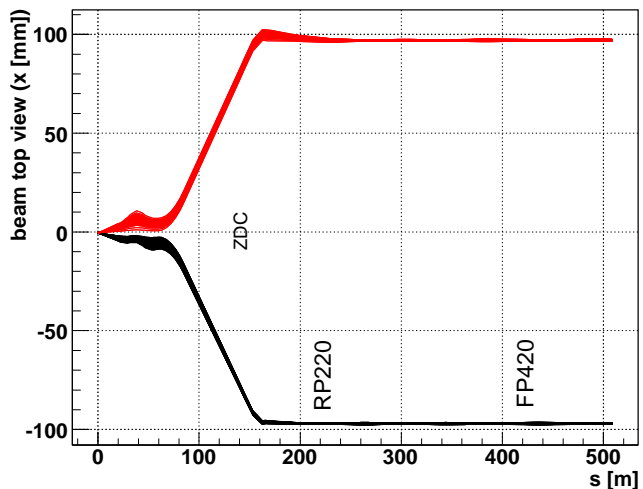
Figure 4: Default location of the very forward detectors, including ZDC and FP420 in the LHC beamline. Incoming (red) and outgoing (black) beams on one side of the interaction point ( s = 0 m). The Zero Degree Calorimeter is located in perfect alignment with the beamline axis at the interaction point, at 140 m, the beam paths are separated. The forward taggers are near-beam detectors located at 220 m and 420 m. Beamline simulation with HECTOR [9].
