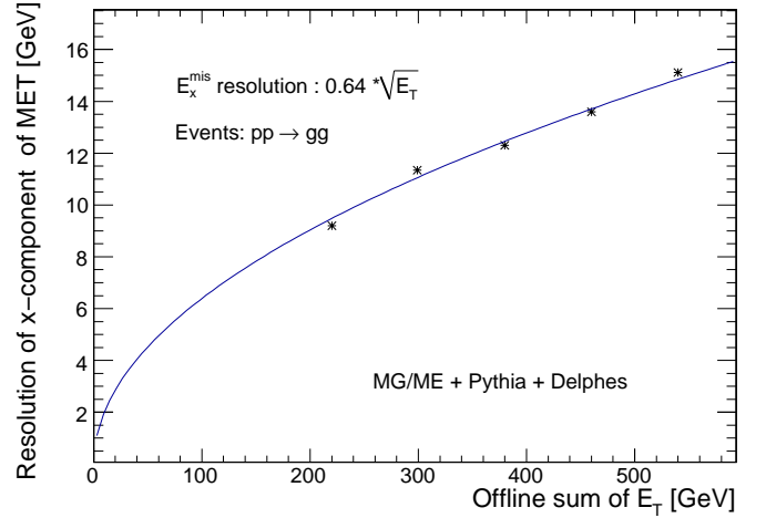
Figure 9: \sigma(E_x^{\text{miss}}) as a function on the scalar sum of all towers ( \Sigma E_T ) for pp \rightarrow gg events.
