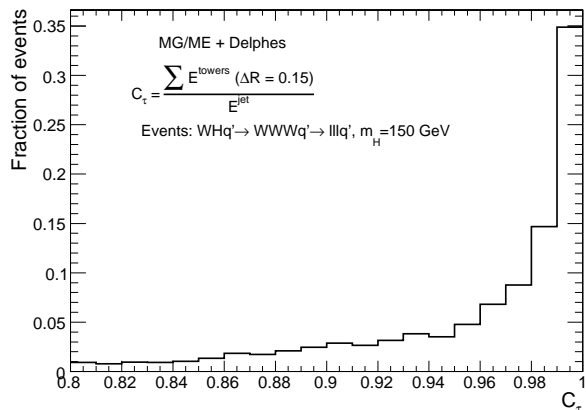
Figure 6: Distribution of the electromagnetic collimation C_\tau variable for true \tau -jets, normalised to unity. This distribution is shown for associated WH photoproduction [15], where the Higgs boson decays into a W^+W^- pair. Each W boson decays into a l\nu_\ell pair, where l = e, \mu, \tau . Events generated with MADGRAPH/MADEVENT [16]. Final state hadronisation is performed by PYTHIA [17]. Histogram entries correspond to true \tau -jets, matched with generator level data.
