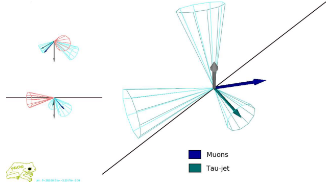
Figure 11: Example of pp(\gamma p \rightarrow Wt)pY event, with t \rightarrow Wb . One W boson decays into a \mu\nu_\mu pair and the second one into a \tau\nu_\tau pair. The surviving proton leaves a forward hemisphere with no hadronic activity. The isolated muon is shown as the blue vector. The \tau -jet is the cone around the green vector, while the reconstructed missing energy is shown in gray. One jet is visible in one forward region, along the beamline axis, opposite to the direction of the escaping proton.
