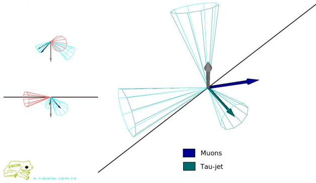
Figure 12: Example of pp(\gamma p \rightarrow W t)pY event. One W boson decays into a \mu \nu_\mu pair and the second one into a \tau \nu_\tau pair. The surviving proton leaves a forward hemisphere with no hadronic activity. The isolated muon is shown as the blue vector. The \tau -jet is the cone around the green vector, while the reconstructed missing energy is shown in gray. One jet is visible in one forward region, along the beamline axis, opposite to the direction of the escaping proton.
