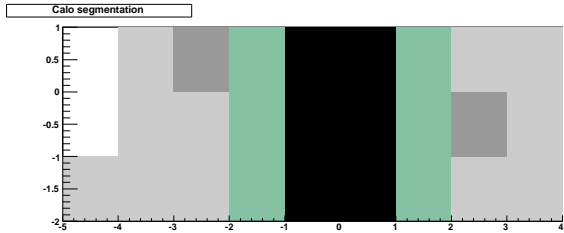
Figure 3: Default segmentation of the calorimeters in the (\eta, \phi) plane. Only the central detectors (ECAL, HCAL and FCAL) are considered.
