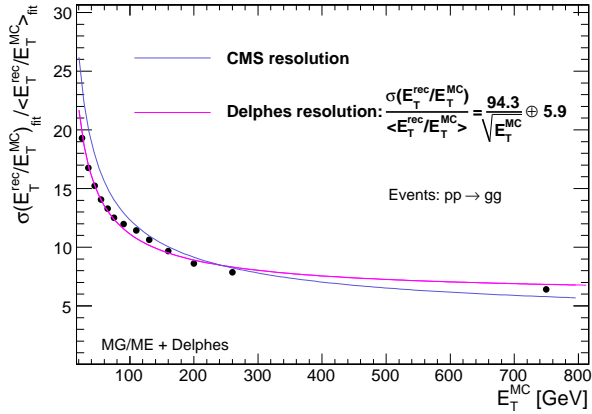
Figure 8: Distribution of the jet transverse energy resolution as a function of the particle-level jet transverse energy. The maximum allowed separation between the DELPHES and the particle-level jets is \Delta R < 0.25 .
