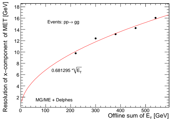
Figure 9: \sigma(E_x^{miss}) as a function on the scalar sum of all towers ( \Sigma E_T ) for pp \rightarrow gg events.
