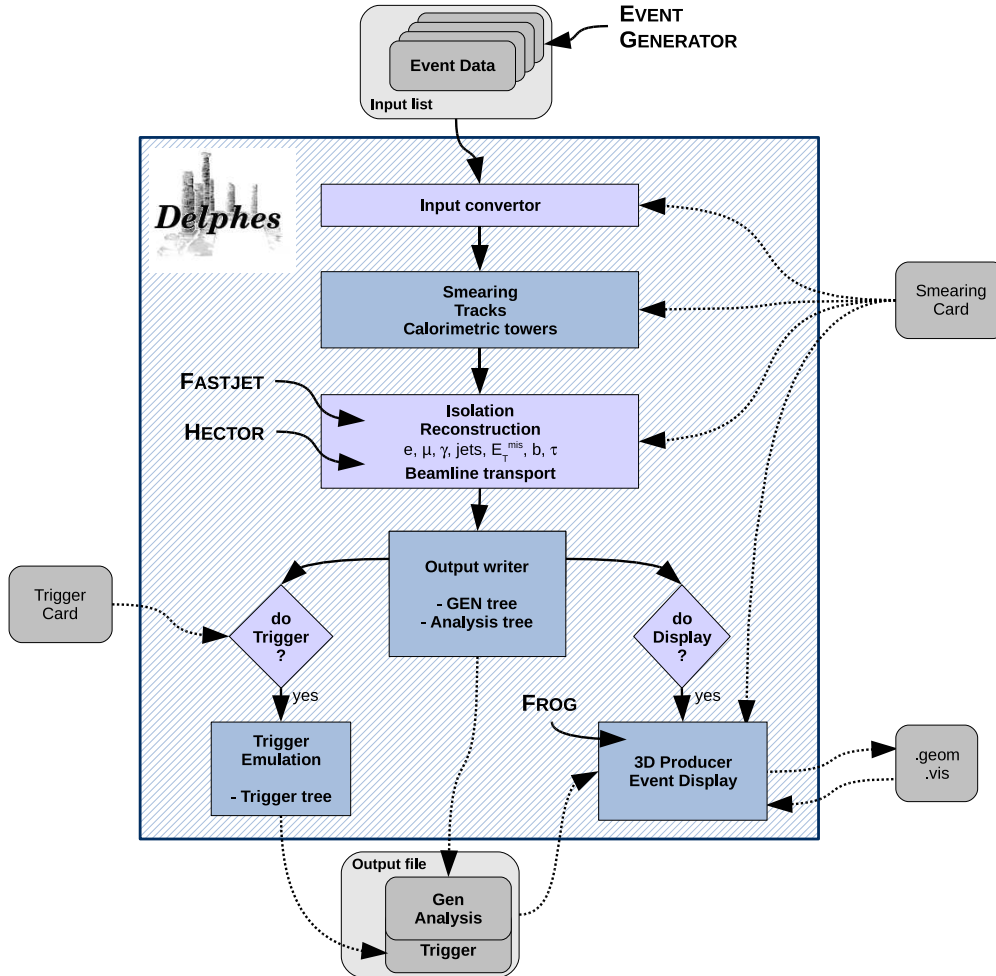
Figure 1: Flow chart describing the principles behind DELPHES. Event files coming from external montecarlo generators are read by a convertor stage. The kinematical variables of the final state particles are then smeared according to the subdetector resolutions. Tracks are reconstructed in a simulated dipolar magnetic field and calorimetric towers sample the energy deposits. Based on these, dedicated algorithms are applied for particle identification, isolation and reconstruction. The transport of very forward particle to the near-beam detectors is also simulated. Finally, an output file is written, including generator level and analysis object data. If requested, a fully parametrisable trigger can be emulated. Optionnally, the geometry and visualisation files for the 3D event display can also be produced. All user parameters are set in the Smearing Card and the Trigger Card .
