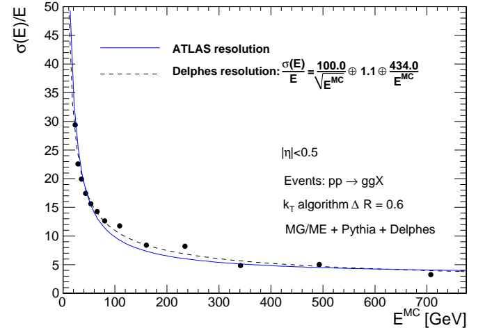
Figure 9: Relative energy resolution of reconstructed jets as a function of the energy of the closest jet of generator-level particles E^{\text{MC}} , in an ATLAS-like detector. The jets are reconstructed with the k_T algorithm with a radius R = 0.6 . The maximal matching distance between mc- and reconstructed jets is \Delta R = 0.2 . Only central jets are considered ( |\eta| < 0.5 ). Dotted line is the fit result for comparison to the ATLAS resolution [8], in blue. The pp \rightarrow gg di-jet events have been generated with MADGRAPH/MADEVENT and hadronised with PYTHIA.
