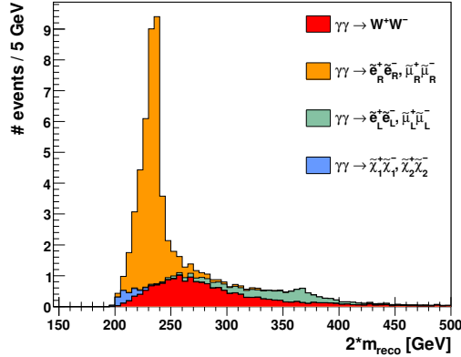
Figure 2: Cumulative distributions of the reconstructed mass 2 * m_{reco} for the integrated luminosity L = 100 \text{ fb}^{-1} assuming no pile-up.
